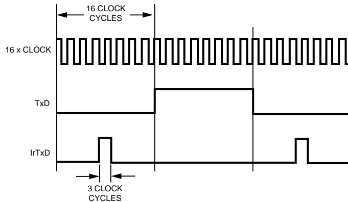
Figure 6.7 IR Transmit.
