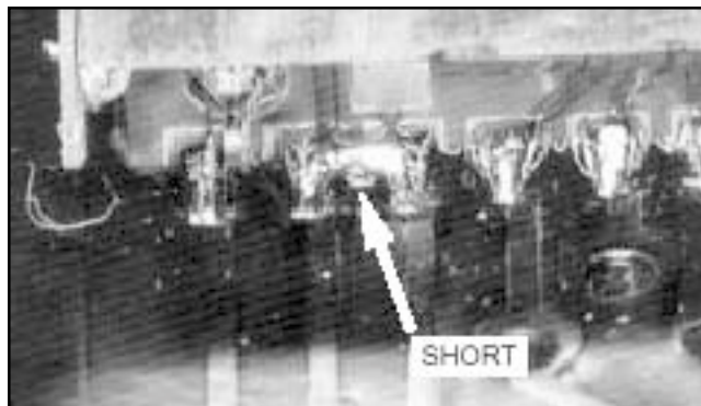
Figure 7.16 Solder Bridging (shorted)
