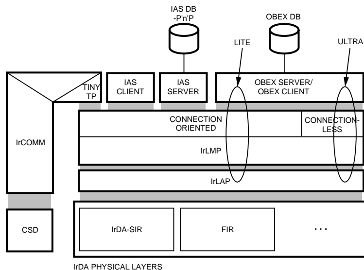
Figure 3.15 IrMC Architecture.
