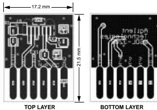
HSDL-3202
